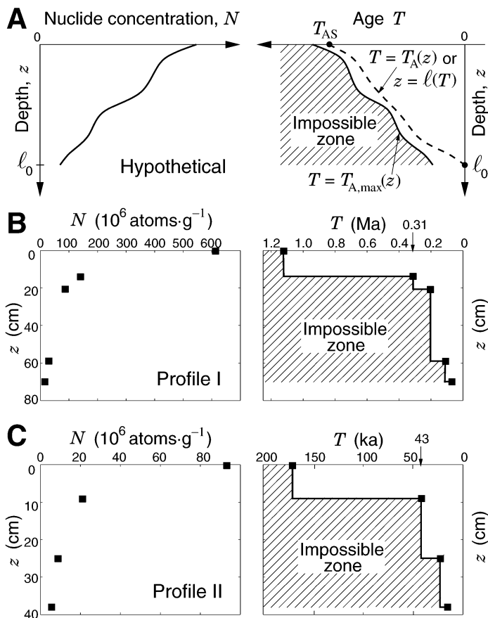
Figure 2. Constraint on past till thickness using ^3\text{He} depth profiles. A: On depth vs. age plot (right panel), till thickness history z = \ell(T) or equivalently accretion age distribution T = T_A(z) (dashed line) must lie outside hatched region, to right of boundary T = T_{A,\max}(z) . This boundary (solid line), given by data (left panel) via equation 8, indicates maximum till thickness at given time. B, C: Application of model in A to profiles I and II. In these cases boundary T_{A,\max}(z) is step like.
