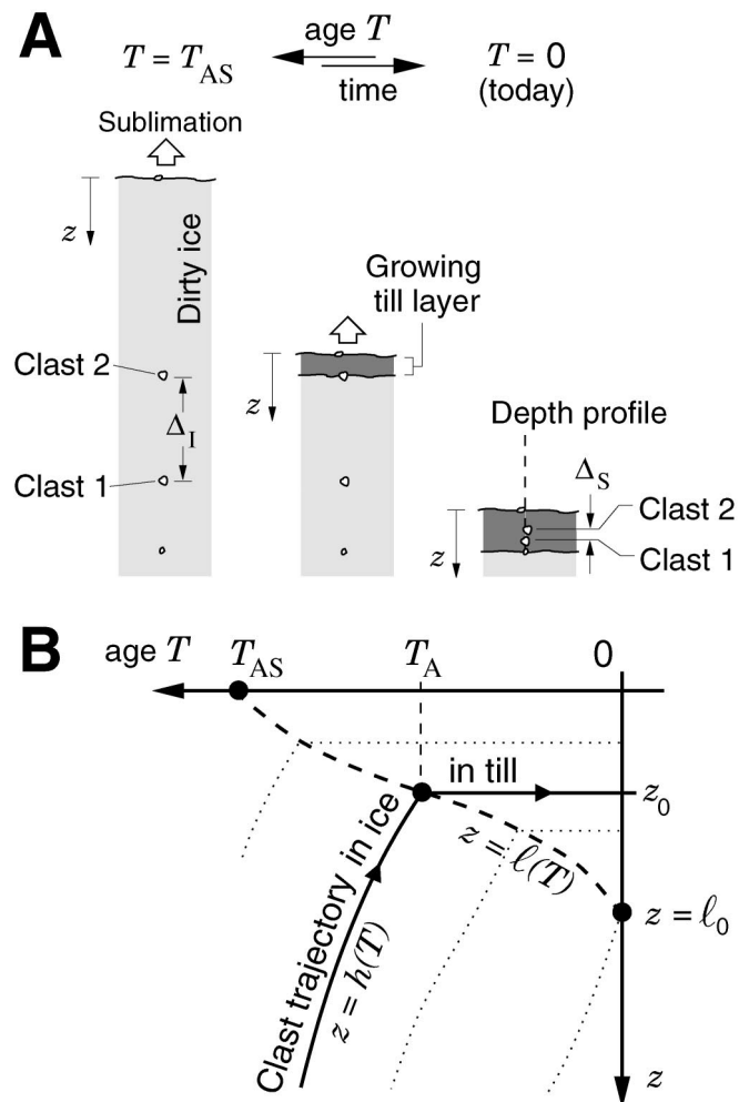
Figure 1. Model of sublimating ice and accreting till with no deformation. A: Processes in reference frame fixed to ice. B: Depth vs. age plot shows processes in reference frame fixed to till surface z = 0 . Heavy dashed line denotes till thickness history \ell . Solid arrowed line is depth history h of clast at z = z_0 today; sublimation uncovers clast until it accretes to till at age T_A , the value of which depends on (and is function of) z_0 . Trajectories of several other clasts are shown dotted.
